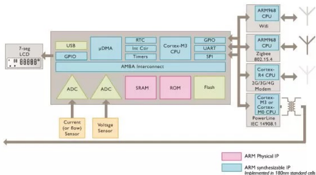
Optimized ARM Smart Meter Block Diagram
